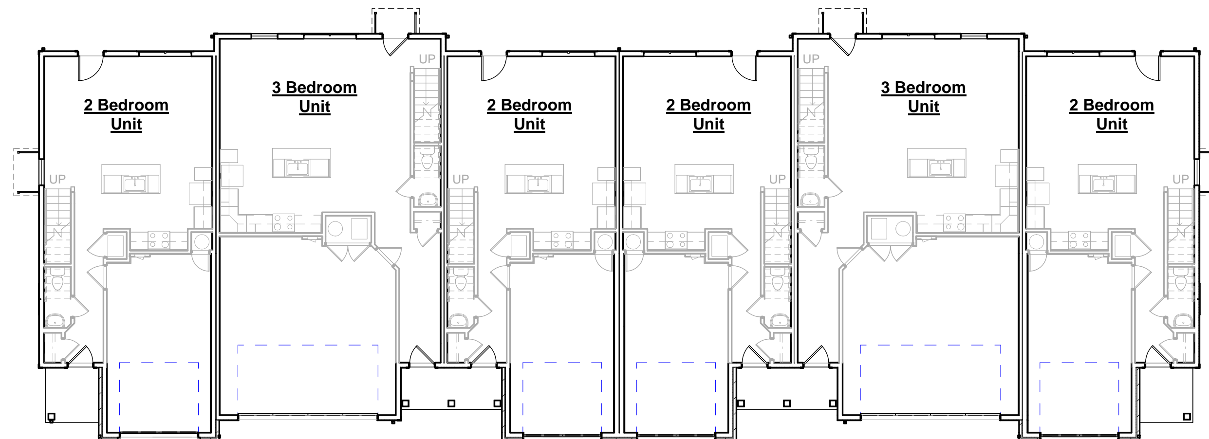
Townhome Building C First Floor Plan 3/32" = 1'-0"
