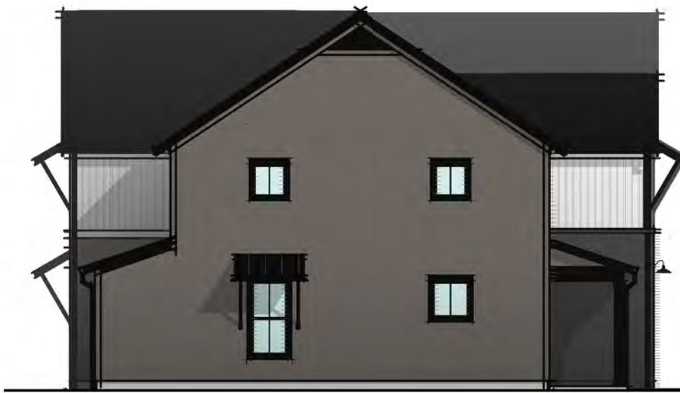
Townhome Building C Left Side Elevation 3/32" = 1'-0"
