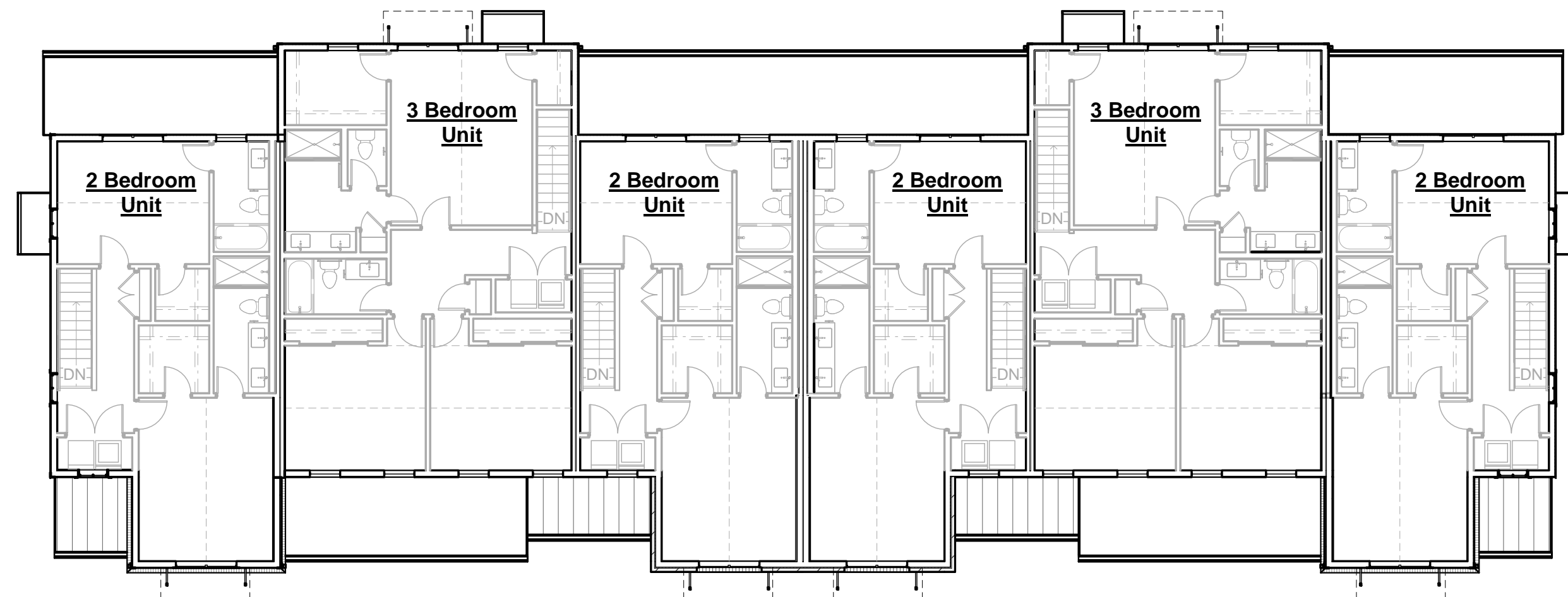
Townhome Building C Second Floor Plan 3/32" = 1'-0"
