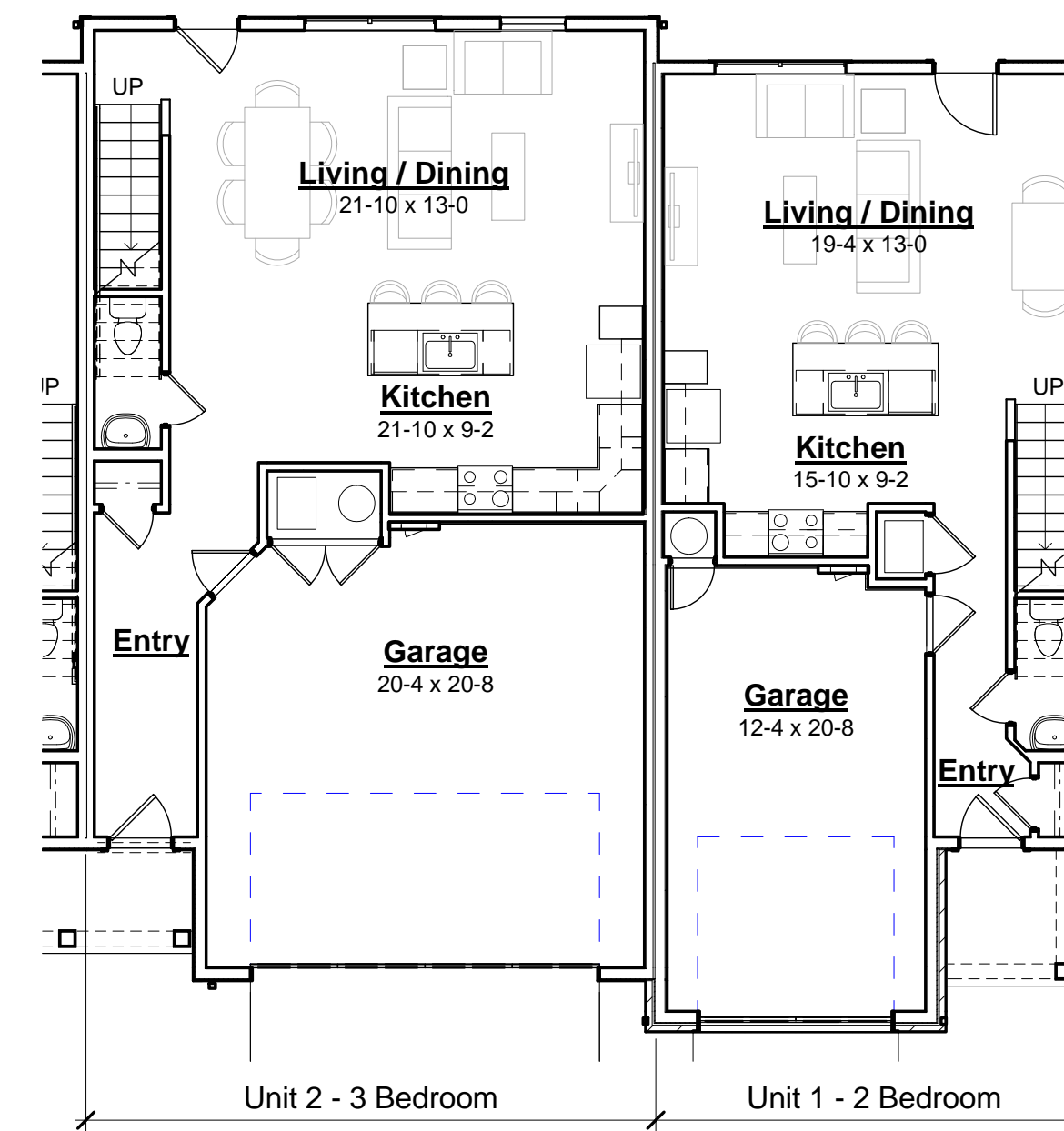
Townhome First Floor Unit Plans 1/8" = 1'-0"
