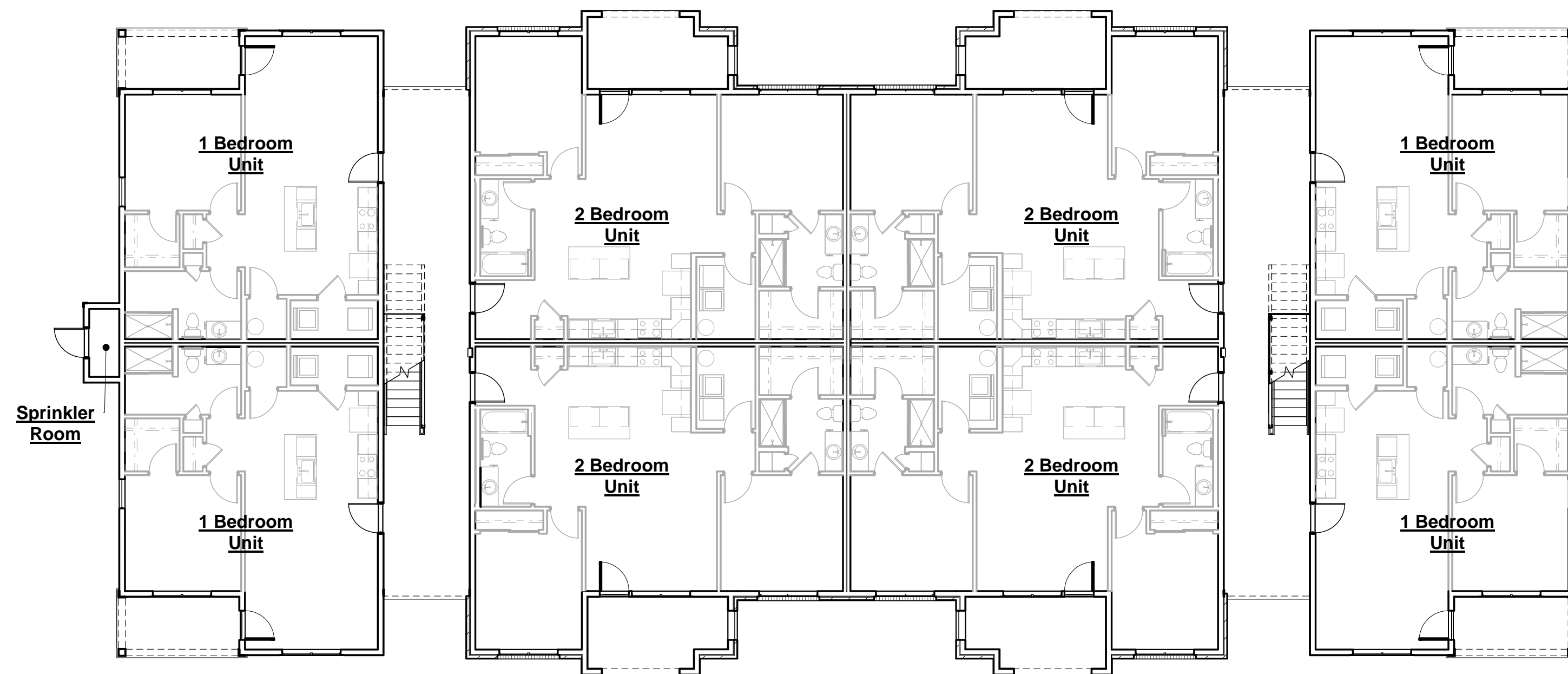
Garden Bldg A - First Floor Plan
